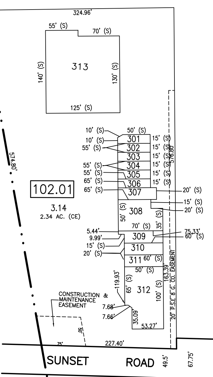
DETAIL "A" 1" = 100'
