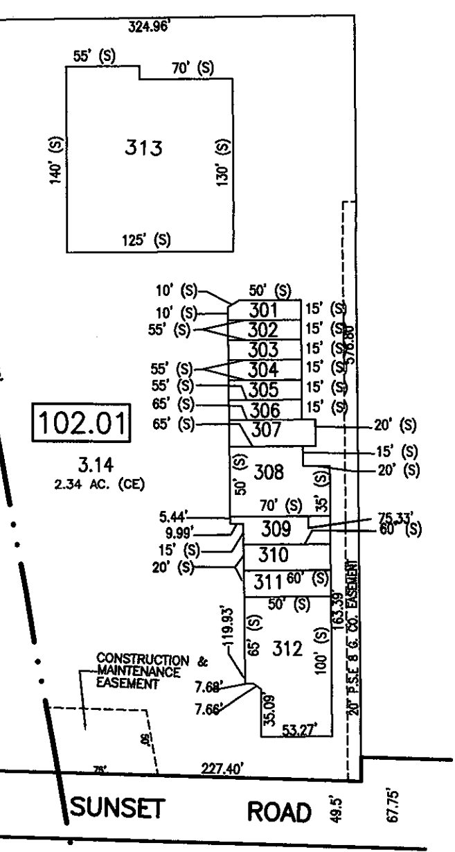
DETAIL "A" 1" = 100'
